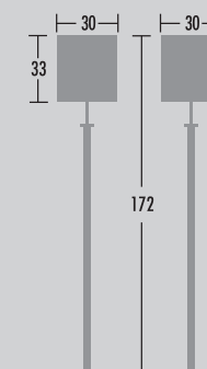
9 VES LP Floor lamp 142-0...-001073 1 x E27
